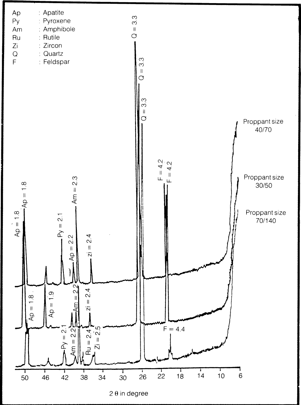
Fig. 8. X-ray diffractometer pattern of Damman sand proppant sizes
