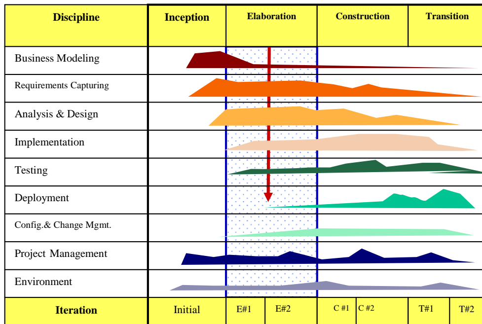
Fig. 3. The overall view of the UP.
