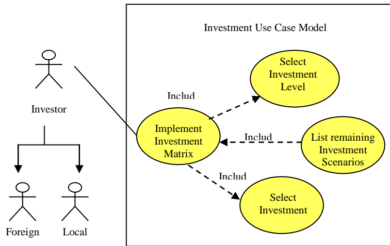
Fig. 4. The use-case model.
