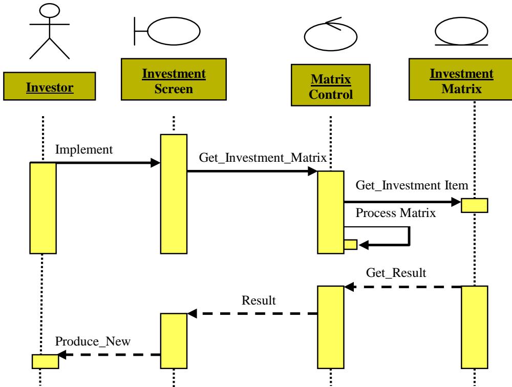
Fig. 5. The sequence diagram.
