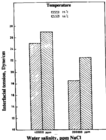
Fig. 10. Interfacial tension between South Geisum crude oil, and sea water and formation water.
