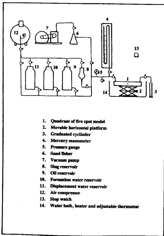
Fig. 1. Schematic diagram of the displacement apparatus
