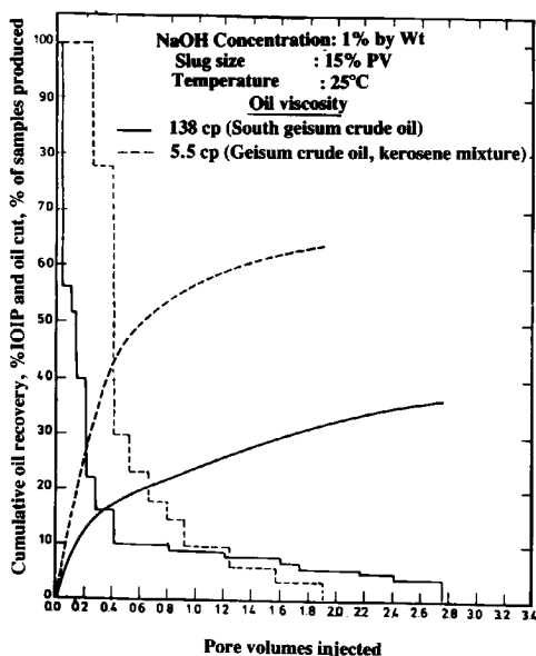
Fig. 14. Effect of oil viscosity on oil recovery by alkaline waterflood
