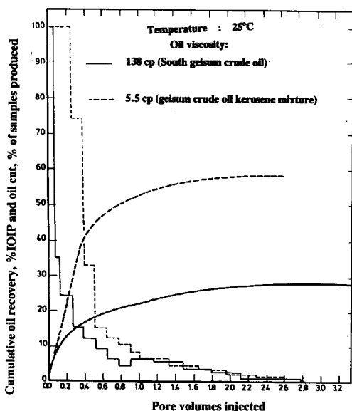
Fig. 13. Effect of oil viscosity on oil recovery by conventional waterflood
