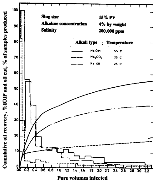
Fig. 11. Effect of temperature and alkali type on oil recovery by alkaline waterflood
