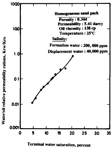
Fig. 2. Water/oil relative permeability ratio versus terminal water saturation.
