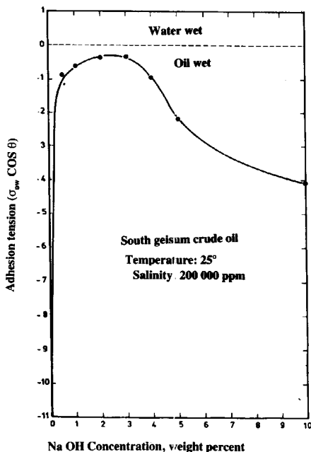
Fig. 7. Adhesion tension ( \sigma_w \cos \theta ) versus NaOH concentration
