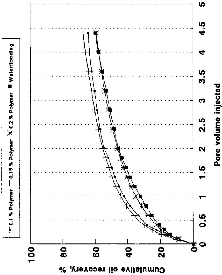
Fig.4 Effect of polymer concentration on oil recovery through parallel horizontal well.
