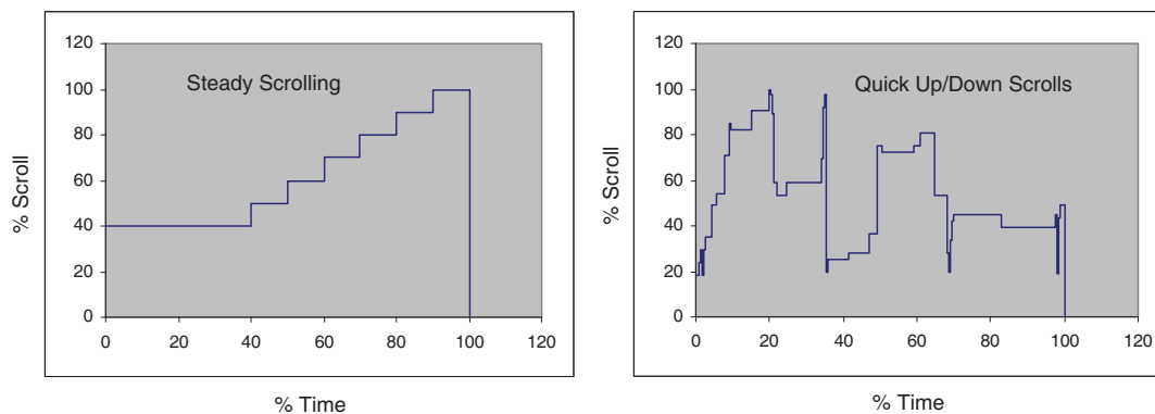
Fig. 3. Typical scroll-time plots for "Steady Scroll Down" and "Quick Up/Down Scroll" patterns.
