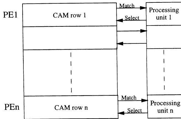
Fig. 4. Associative processor architecture.
