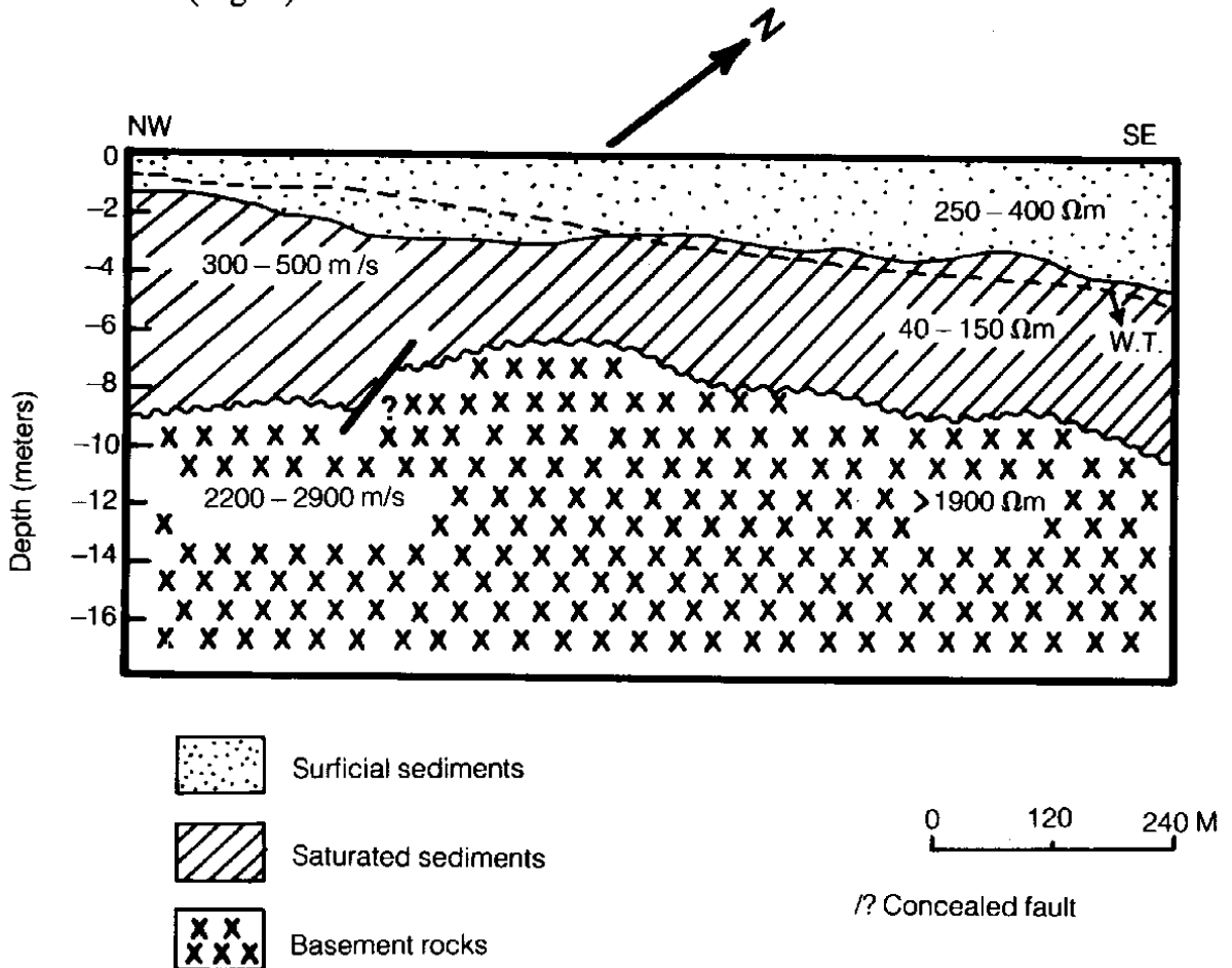
Fig. 9. Generalized subsurface geological section. Geological boundaries are based on resistivity and seismic velocity contrasts.
