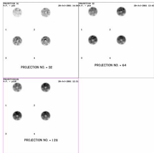
Fig. 3. Transaxial image reconstruction of a cylindrical phantom filled with Tc-99m with different projection numbers.
