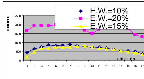
Fig. 6. Shows the counts profile with respect to position for different energy window width.
