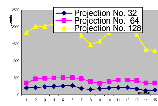
Fig. 4. The counts profile with respect to position for different projection numbers.
