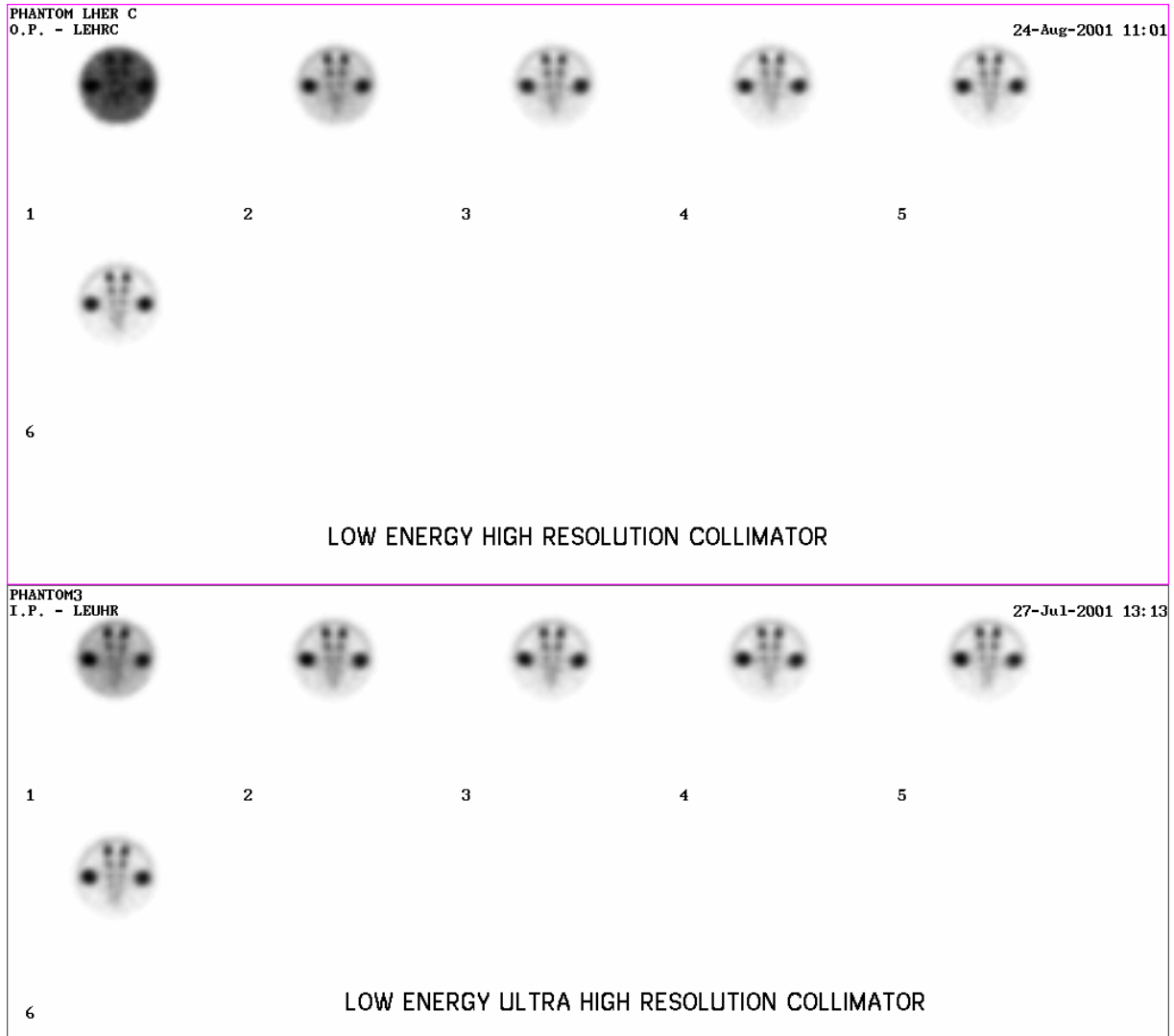
Fig. 7. Transaxial image reconstruction of a cylindrical phantom filled with Tc-99m using different types of collimators (LEUHRC and LEHRC).
