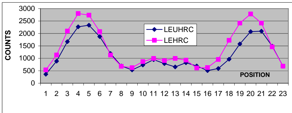
Fig. 8. Shows the counts profile with respect to position for different type collimators.
