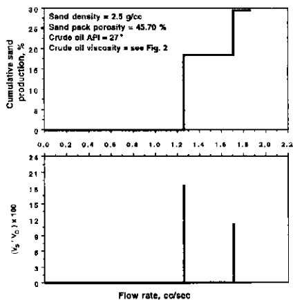
Fig. 20. Sand/Heavy oil ratio (by volume) and cumulative sand production % versus flow rate at CP - 0.0 MPa.
