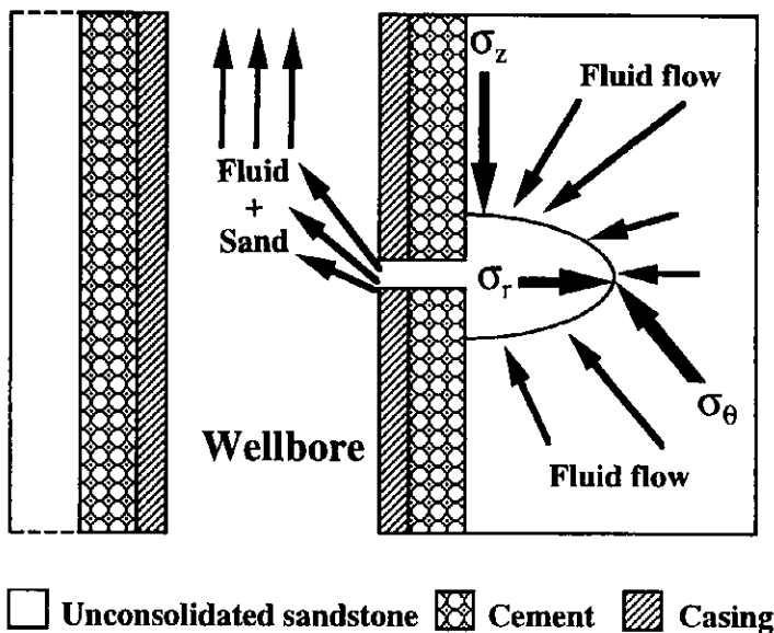
Fig.1. Sand arch failure mechanism [1].
