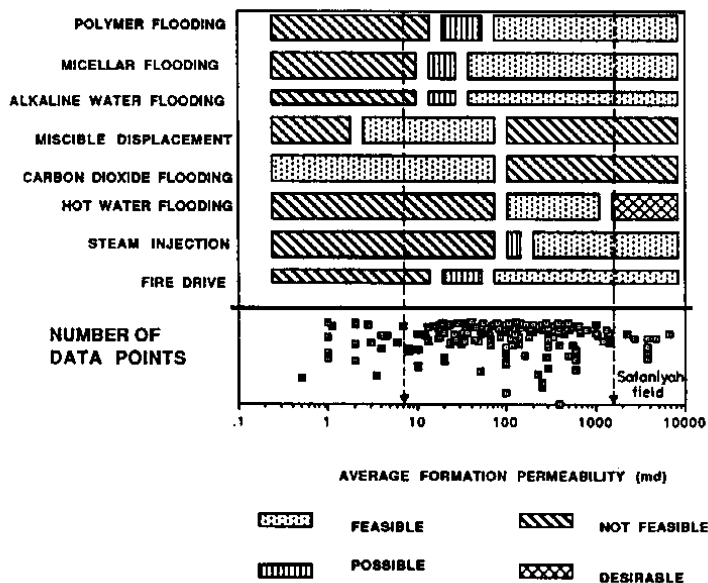
Fig. 5. Saudi reservoirs formation permeability guides for applying e.o.r. methods
