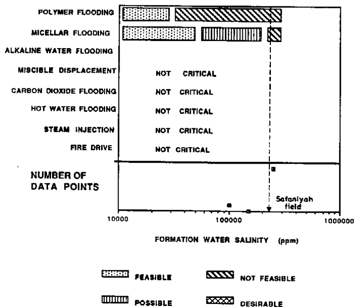
Fig. 4. Feasibility of e.o.r. methods to Saudi formations water salinity
