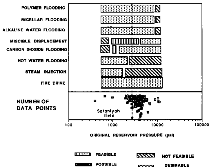
Fig. 3. Original Saudi reservoirs pressure limitation for different e.o.r. methods
