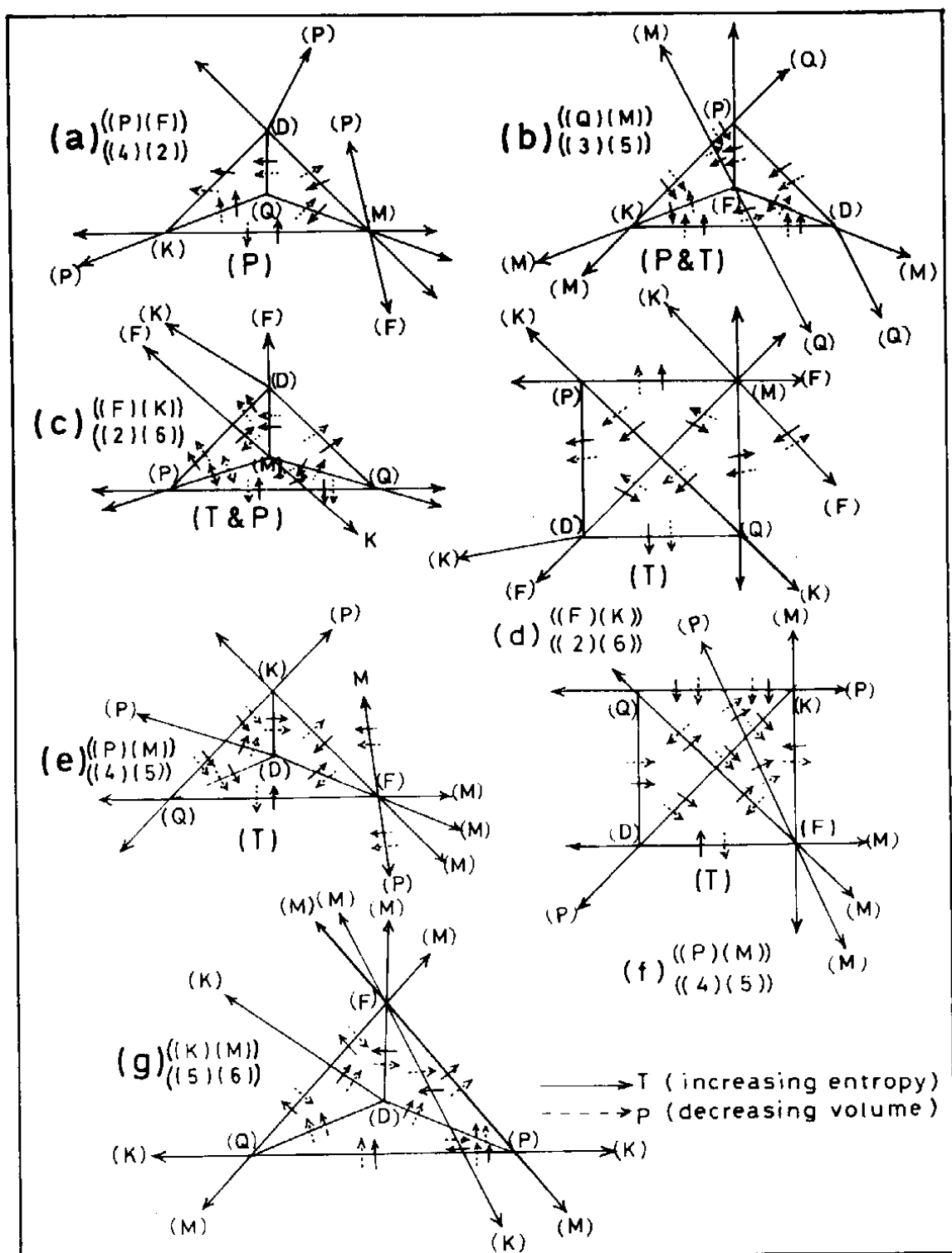
Fig. 6. Set of seven nets of maximum closure oriented according to thermodynamic data of Table 3(2). The elimination of a net on the basis of P and/or T arrows is indicated by (P), (T), or (P & T) beneath each net.
