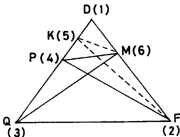
Fig. 3. Ternary degenerate chemography for the system KASH corresponding to T 49 of [4].
