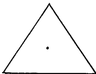
Fig. 4. First permissible net topology in the degenerate chemography of the system KASH (a triangle with a central invariant point).
