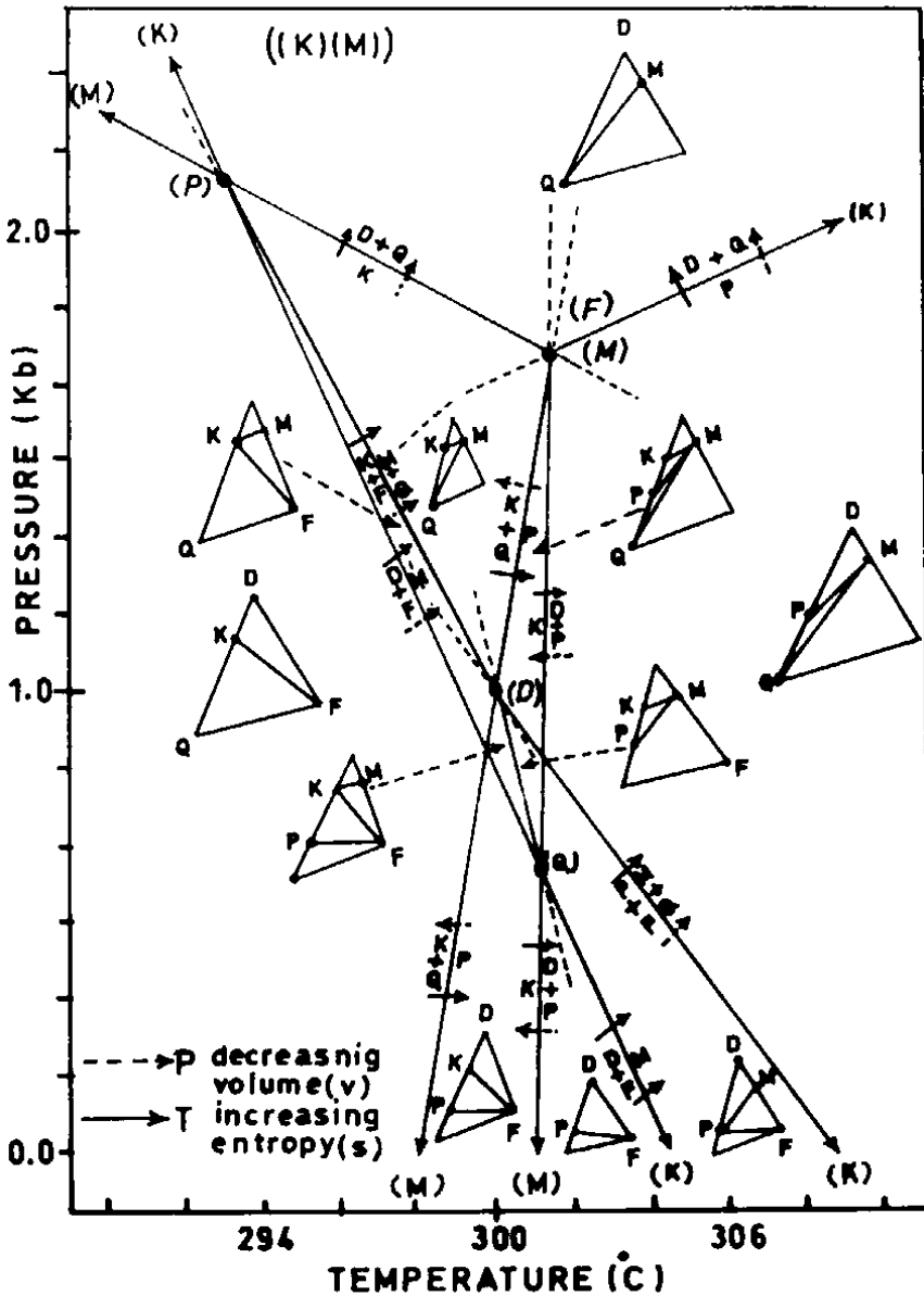
Fig. 7. Topology of the oriented partially-closed net of maximum closure in the system KASH [net ((K)(M)) of Fig. 6g].
