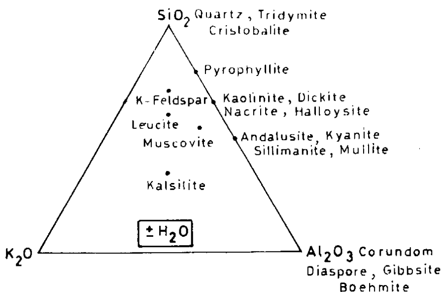
Fig. 1. Triangular composition diagram in the system KASH ( \text{K}_2\text{O} - \text{Al}_2\text{O}_3 - \text{SiO}_2 - \text{H}_2\text{O} ), \mu_{\text{H}_2\text{O}} is held constant.
