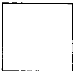
Fig. 5. Second permissible net topology in the degenerate chemography of the system KASH (a square without invariant point in the center).
