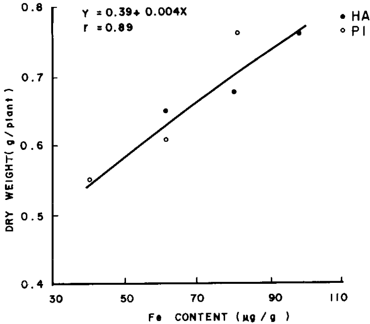
Fig. 2. Relationship between iron content and dry weight of soybean plant top
