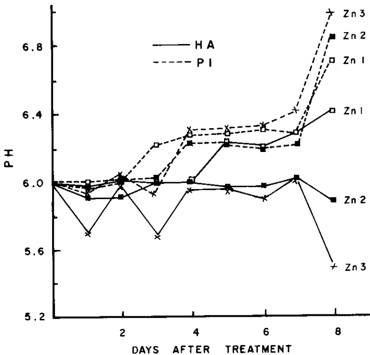
Fig. 1. pH of solution cultures as affected by soybean genotypes and zinc level
