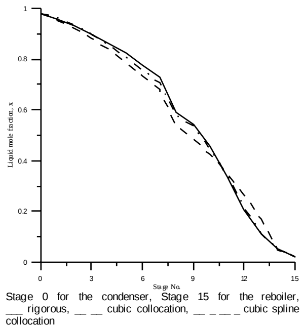
Fig. 2. Composition profile in the distillation column.
