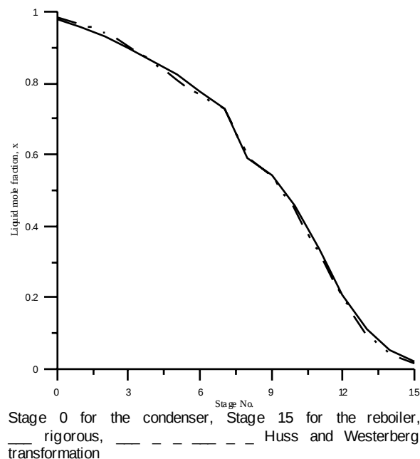
Fig. 3. Composition profile in the distillation column.
