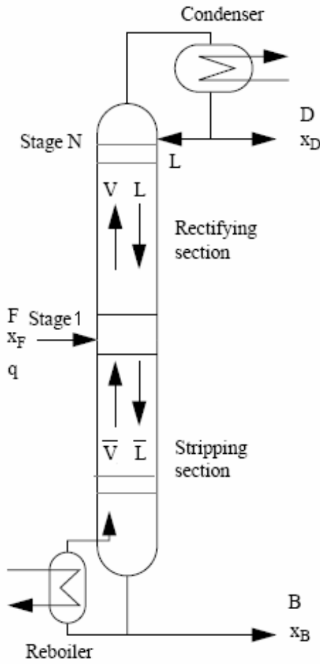
Fig. 1. A two-product distillation column.
