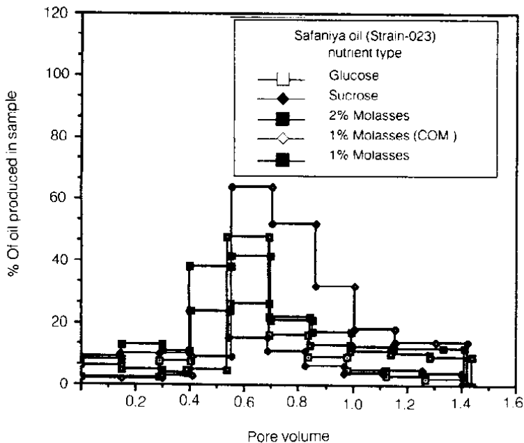
Fig. 2. Effect of nutrient type on % of oil produced in sample.
