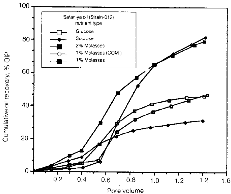
Fig. 3. Effect of nutrient type on cumulative oil recovery.
