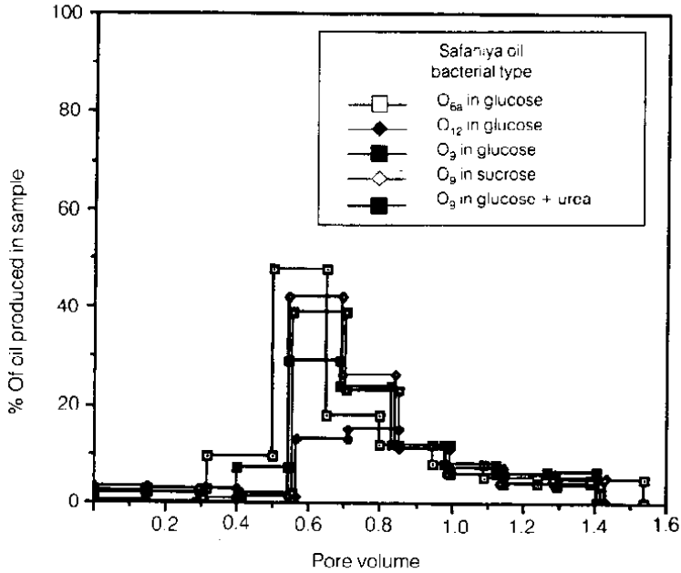
Fig. 6. Effect of bacterial type on % of oil produced in sample.
