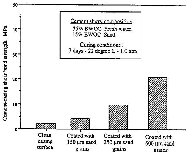
(b) Casing roughness-shear bond strength relationship.
