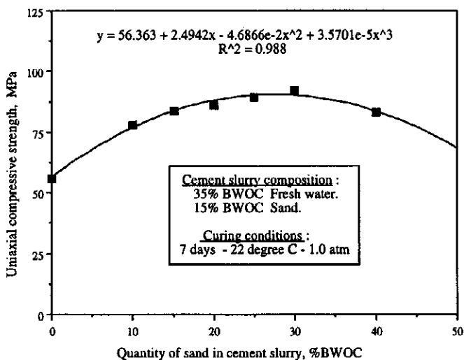
Fig. 2. Effect of sand addition on cement compressive strength.
