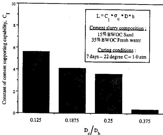
Fig. 13. Effect of cement sheath strength and casing size to hole size ratio on cement supporting capability.
