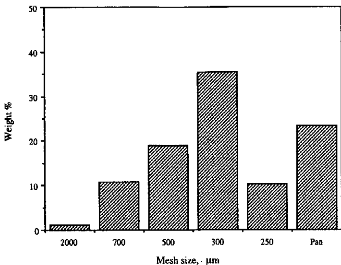
Fig. 1. Granulometric analysis of Thumama sand.
