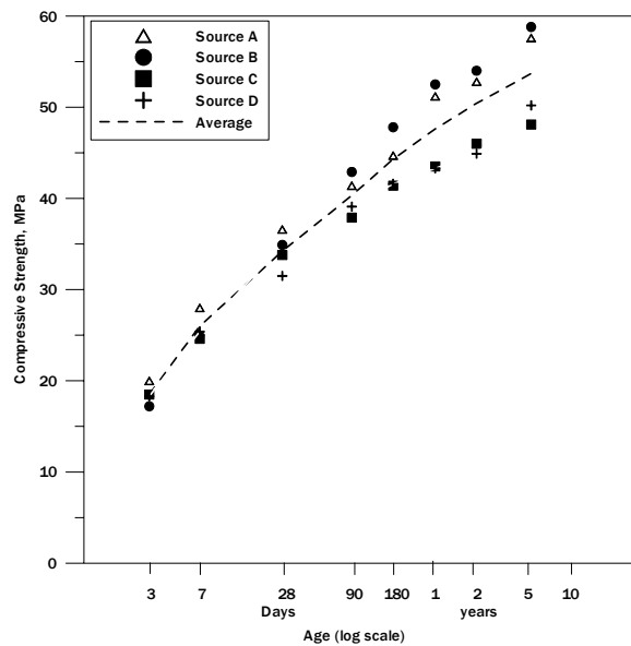
Fig. 2. Strength development of concrete made with Type I cement.
