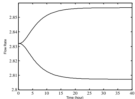
Fig. 4. Output flow rate Q_o(t) \text{ m}^3/s for N = 985 \pm 10\% rpm square wave speed variation.
