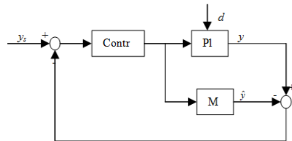
Fig. 1. Predictive control structure.
