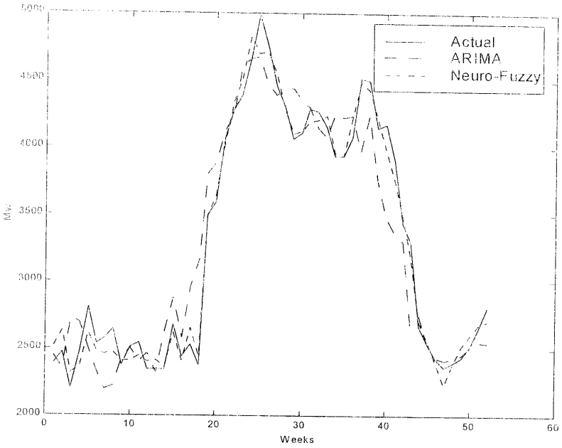
Fig. 9. Forecasting 1997 weekly peak loads for Riyadh.
