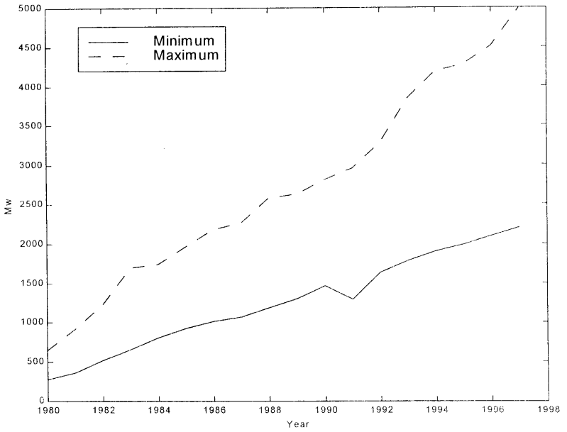
Fig. 1. Minimum and maximum peak loads (1980-1997).
