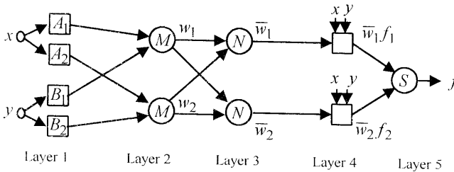
Fig. 5. Equivalent ANFIS architecture [11].
