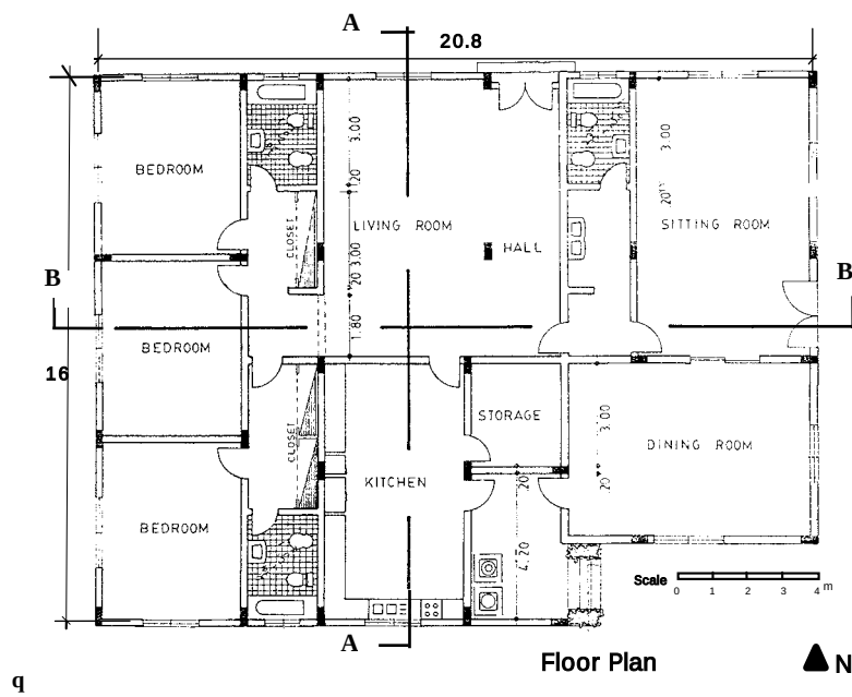
Fig. 4. Floor plan of the one-story house.
