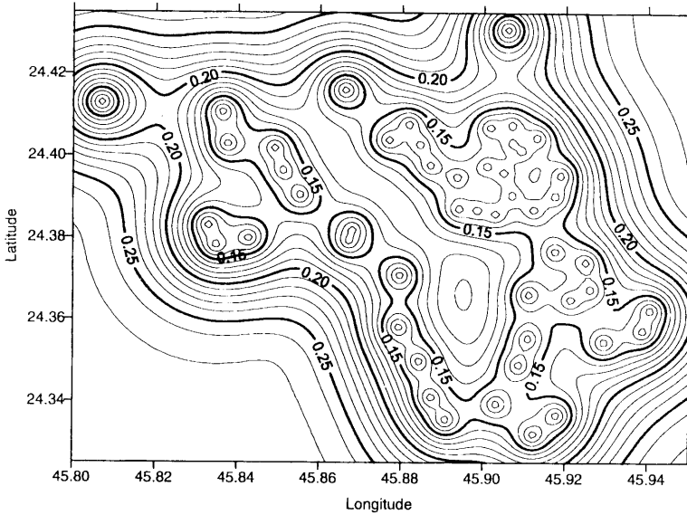
Fig. 5. Isarithmic map of kriging variance ( \text{mS cm}^{-1} ) 2 .
