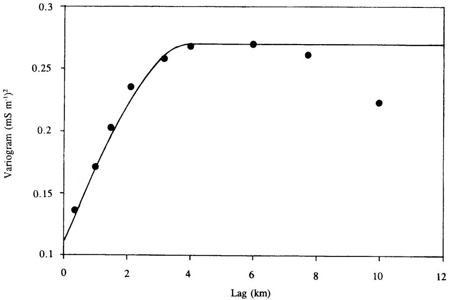
Fig. 3. Plot of experimental variograms \text{(mS cm}^{-1}\text{)}^2 vs lag (km).
