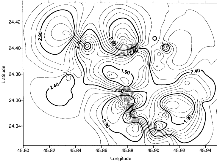
Fig. 4. Isarithmic map of groundwater salinity ( \text{mS cm}^{-1} ).
