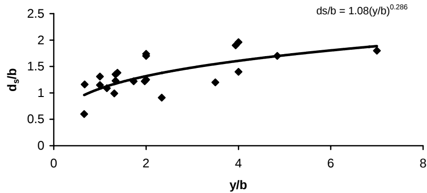
Fig. 3. Variation of flow depth with local scour depth.
