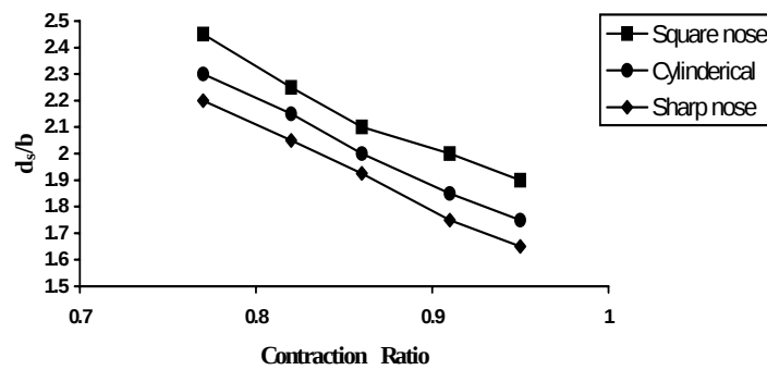
Fig. 7. Effect of the contraction ratio on the local scour depth.
