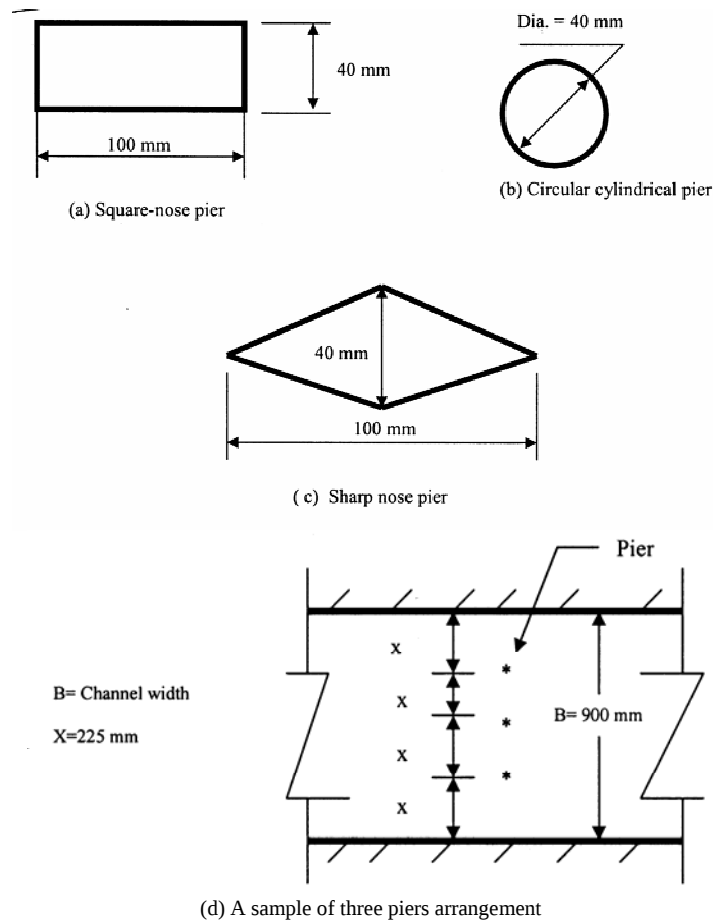
Fig. 2. Shapes, dimensions and arrangements of the piers used in the physical model.
