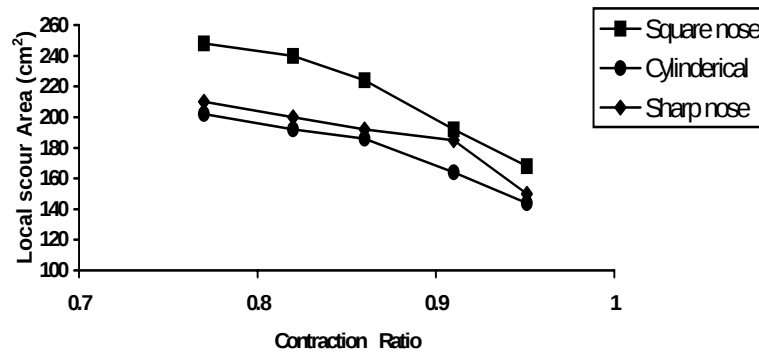
Fig. 8. Effect of the contraction ratio on the size of local scour area.
