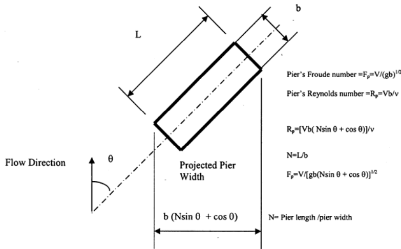
Fig. 1. Geometry of square nose skewed pier.
