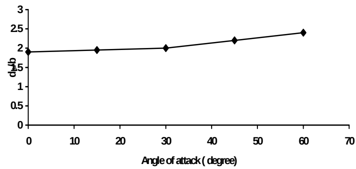
Fig. 6. Effects of pier inclination on local scour depth.
