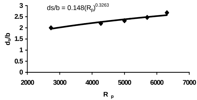
Fig. 5. Variation of pier's Reynolds number with local scour depth.
