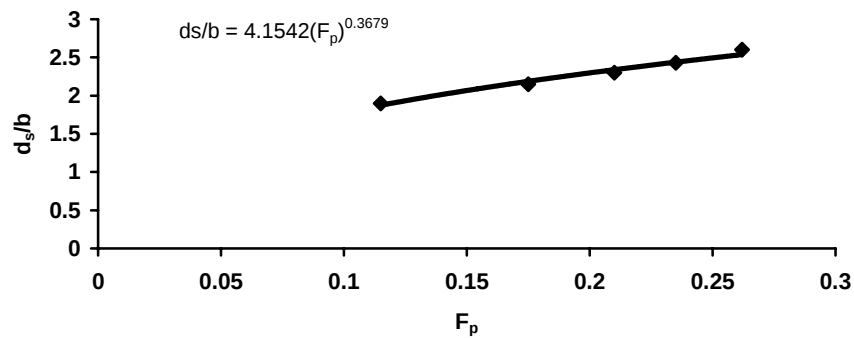
Fig. 4. Variation of Pier Froude number with local scour depth.
