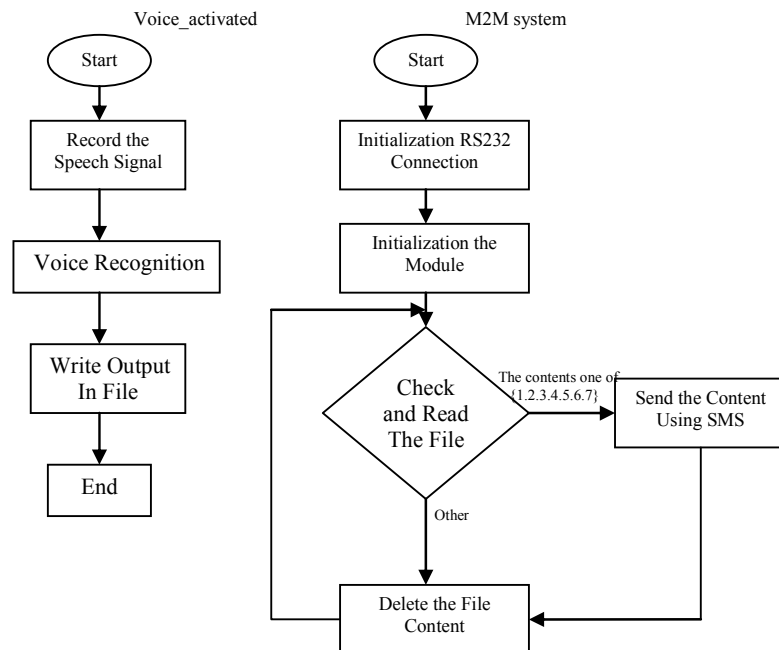
Fig. 7. Flowchart of voice-activated and M2M software implementation.
