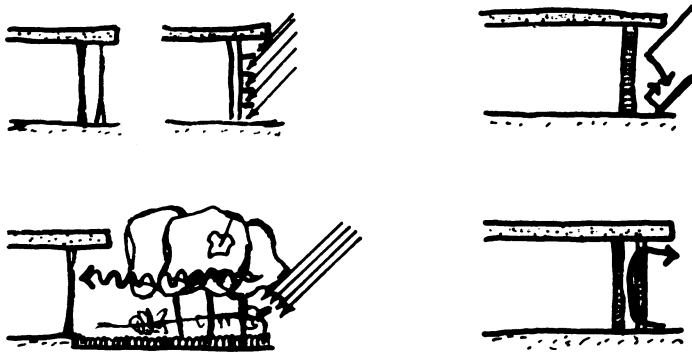
Fig. 6. Shading devices, cavity walls, roof with air space in between will provide a resistance to heat flow [9].
