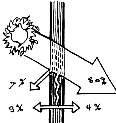
Fig. 15. Solar radiation enters through glazed areas which transmit solar or short-wave radiation with very little loss in heat energy. By greenhouse effect, the heat enters through glazed areas in trapped and can increase the indoor temperature to far above that of the air outdoors [6, p.41].
