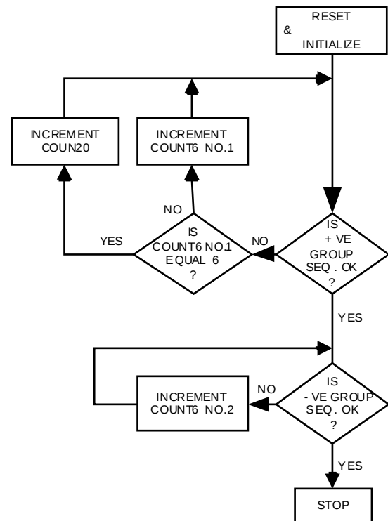
Fig. 3. Flow chart for the proposed scanning system.
