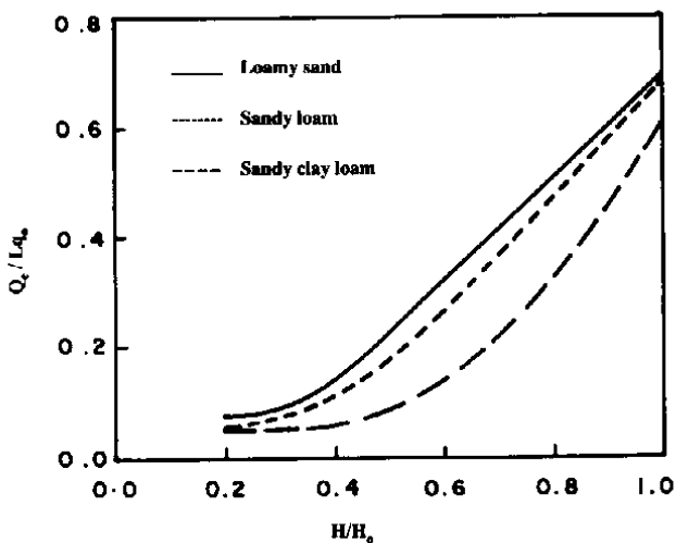
Fig. 6. Evaporation ratio versus intermediate head ratio.
