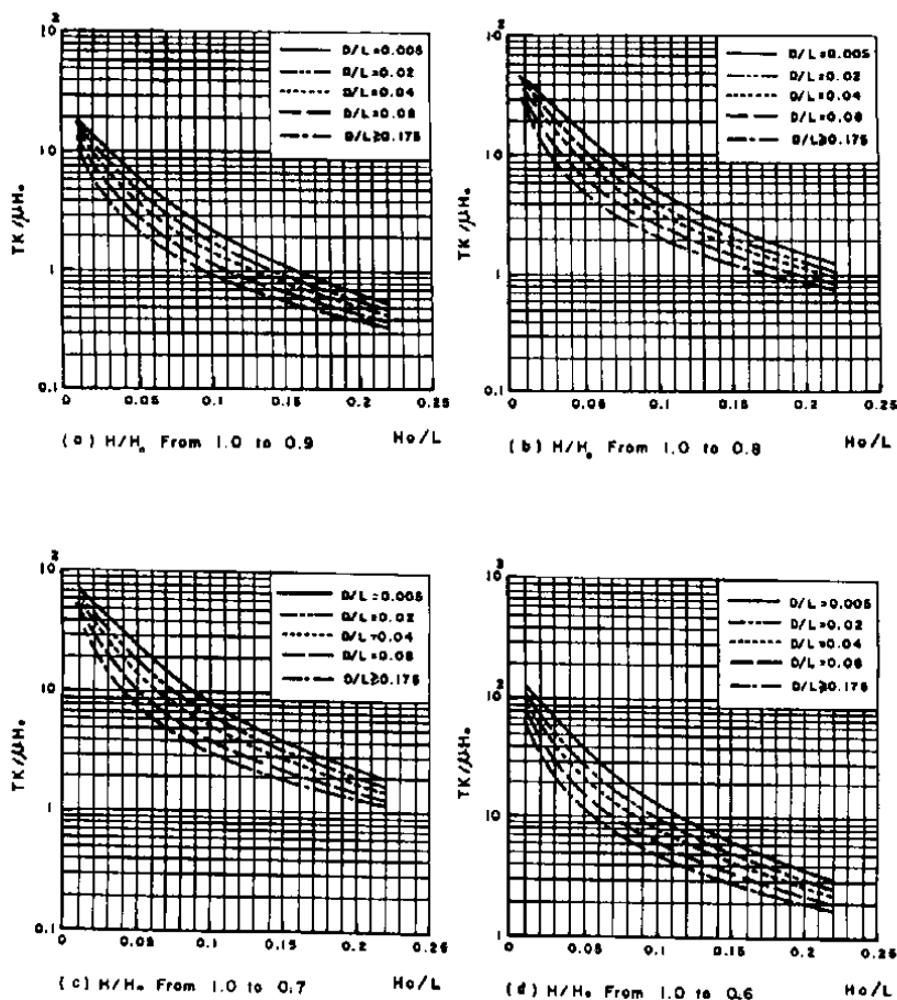
Fig. 9. Drain spacing design chart for sandy clay loam
