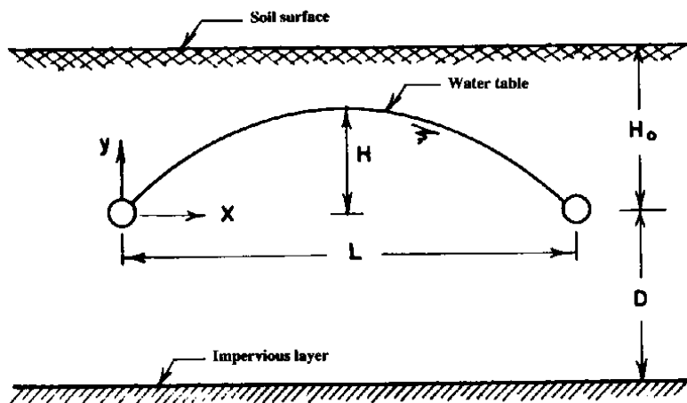
Fig. 1. Definition sketch.
