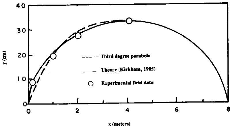
Fig. 2. Experimental field data compared with theory (Kirkham, 1958) and the third degree parabola.
