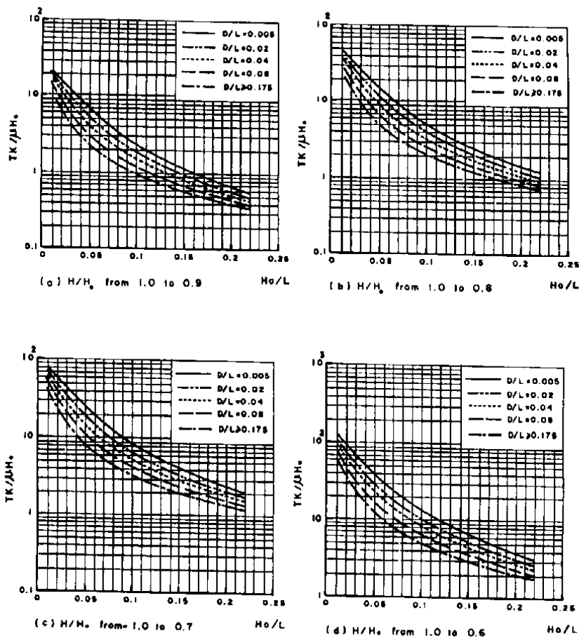
Fig. 7. Drain spacing design chart for loamy sand.
