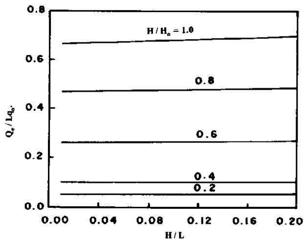
Fig. 4. Evaporation ratio versus water table height ratio for sandy loam.
