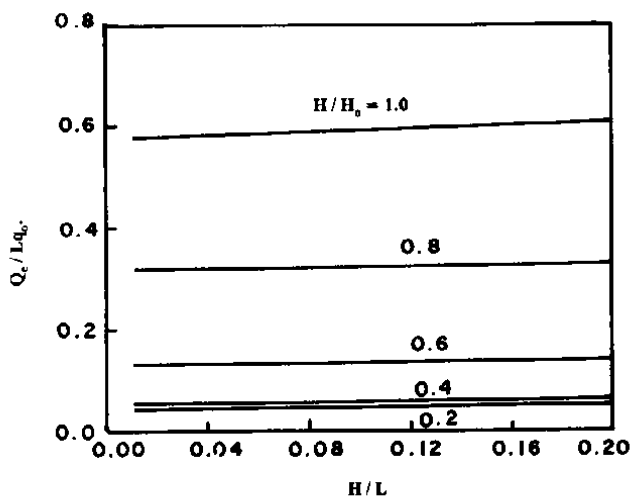
Fig. 5. Evaporation ratio versus water table height ratio for sandy clay loam.
