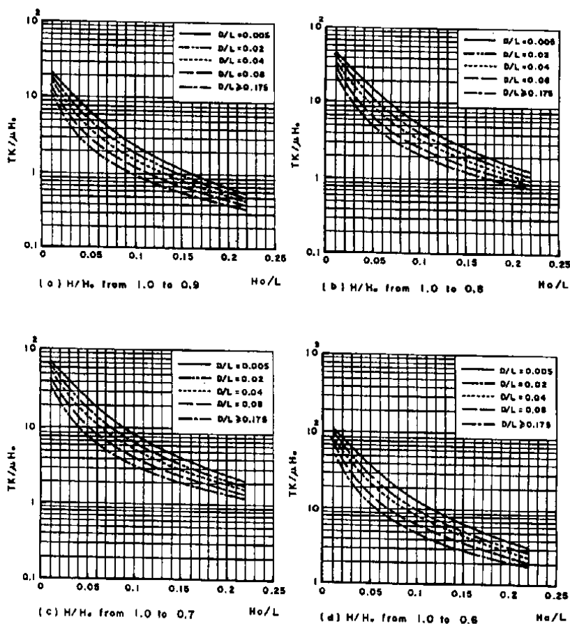
Fig. 8. Drain spacing design chart for sand clay loam.
