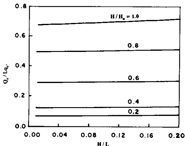
Fig. 3. Evaporation ratio versus water table height ratio for loamy sand.
