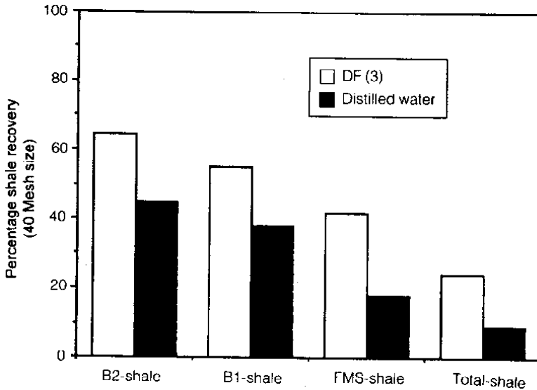
Fig. 11. Dispersibility test result for various types of shale.
