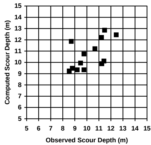
Fig. 4. Comparison of measured and computed scour depths using Jain and Fisher formula.
