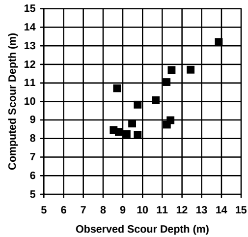
Fig. 2. Comparison of measured and computed scour depths using Melville and Sutherland formula.
