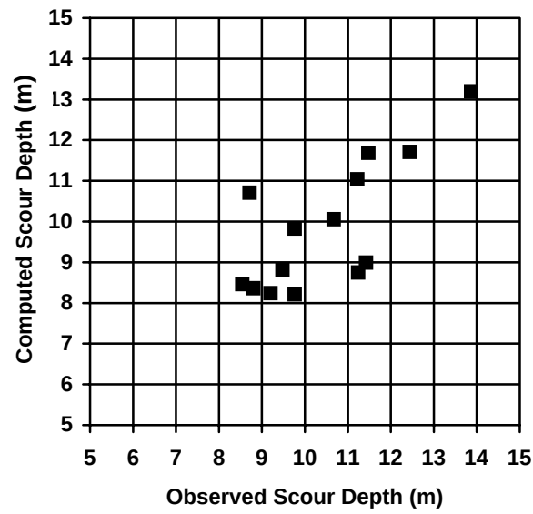
Fig. 1. Comparison of measured and computed scour depths using CSU formula.
