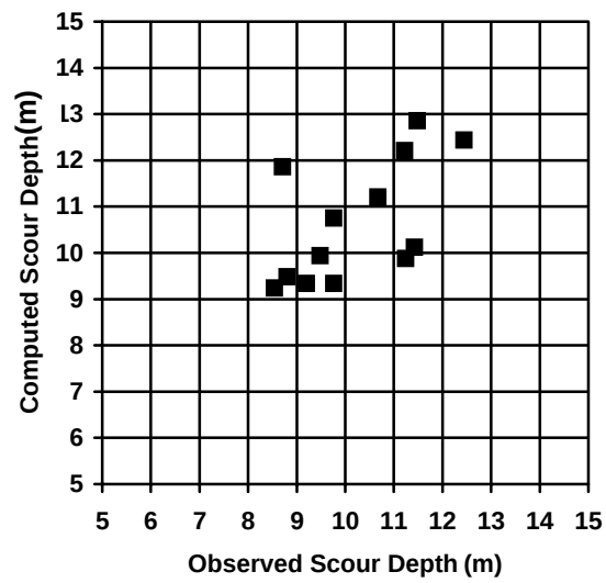
Fig. 3. Comparison of measured and computed scour depths using Lauren and Toch formula.
