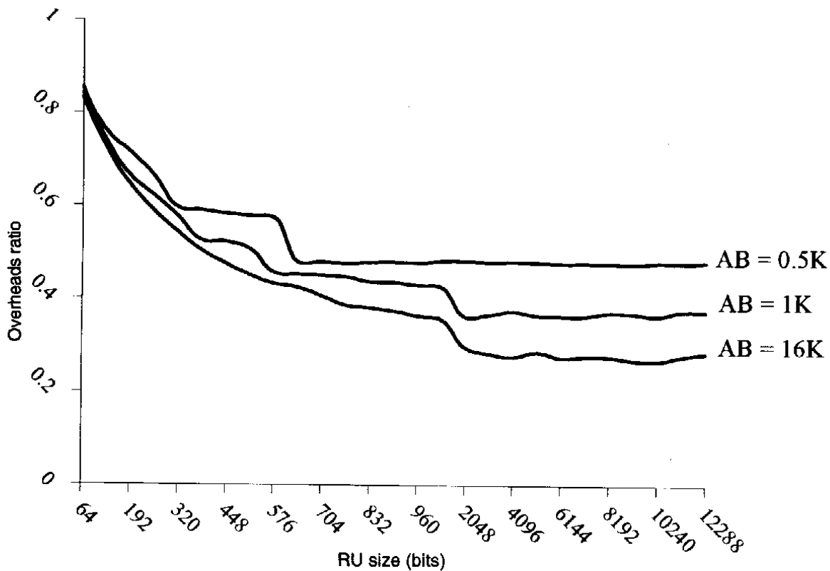
Fig. 4. The overheads ratio versus the RU size for different values of AB. (Mean = 1K, P=1E-5).
