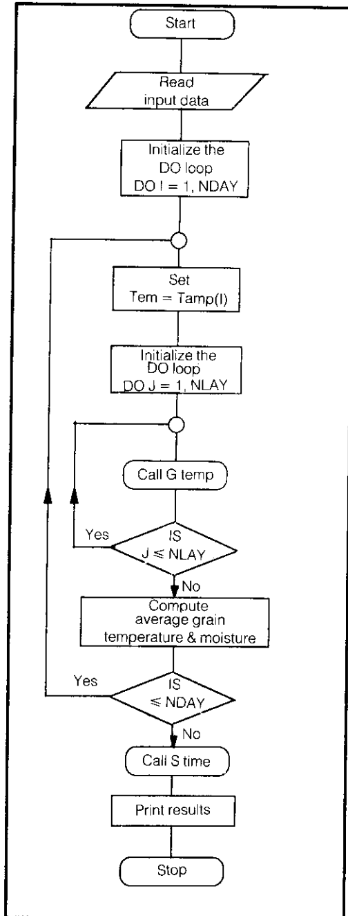
Fig. 2. Storage model flowchart.
