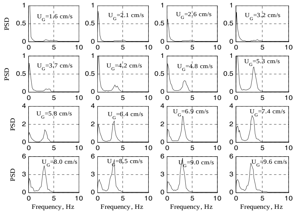
Fig. 7. Spectral density for 5% polyethylene using 100 Hz sampling frequency.
