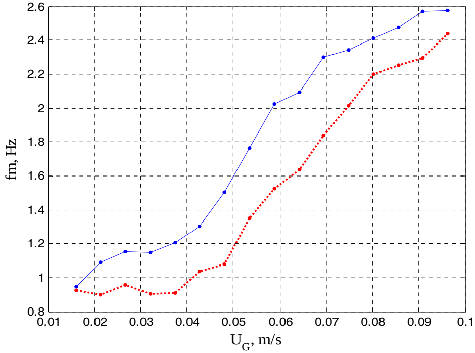
Fig. 8. Average spectral frequency; (dotted) water, (solid) 5% polyethylene.
