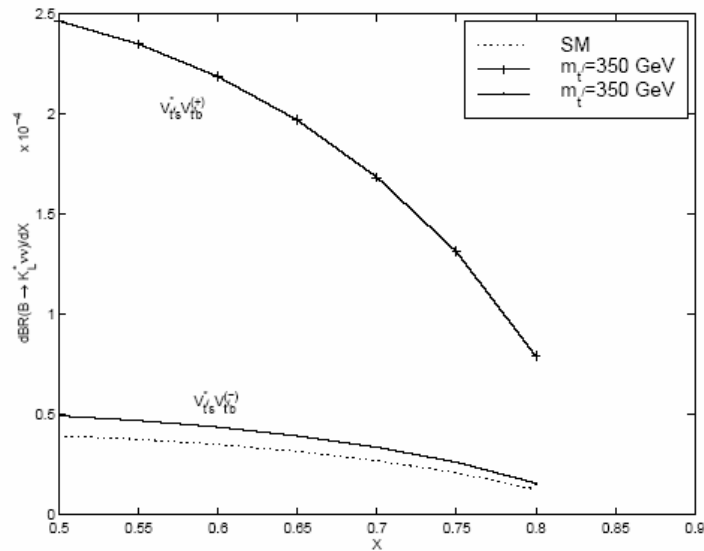
Fig. 2. The dependence of the differential of the BR of the decay B \rightarrow K^* \nu \bar{\nu} on the missing-energy fraction x at fixed value of m_t = 350 GeV when K^* is polarized longitudinally.
