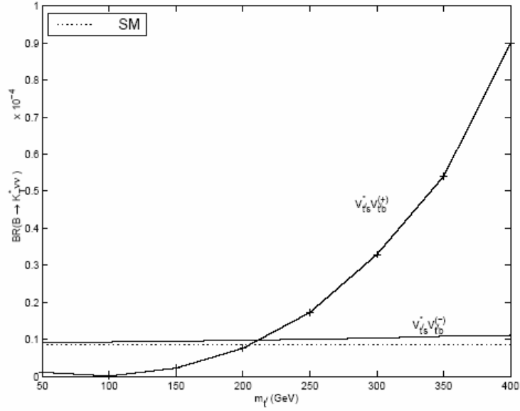
Fig. 6. The dependence of the differential of the BR of the decay B \rightarrow K^* \nu \bar{\nu} on the fourth up-like quark mass m_{t'} , when K^* is polarized transversely.
