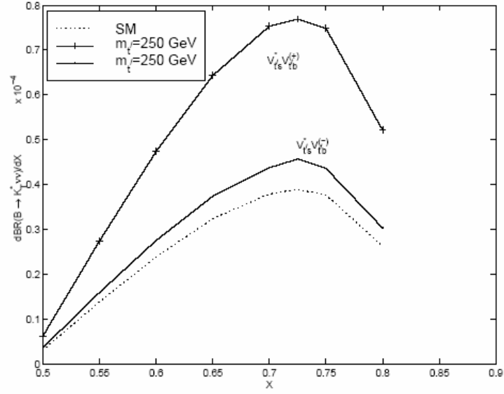
Fig. 3. The dependence of the differential of the BR of the decay B \rightarrow K^* \nu \bar{\nu} on the missing-energy fraction x at fixed value of m_{t'} = 250 GeV when K^* is polarized transversely.
