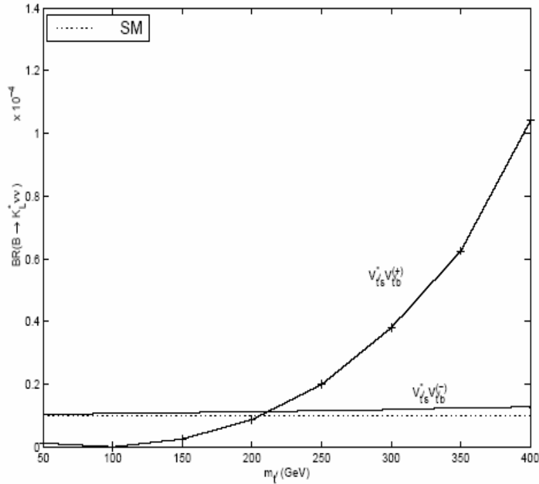
Fig. 5. The dependence of the differential of the BR of the decay B \rightarrow K^* \nu \bar{\nu} on the fourth up-like quark mass m_{t'} when K^* is polarized longitudinally.
