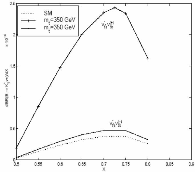
Fig. 4. The dependence of the differential of the BR of the decay B \rightarrow K^* \nu \bar{\nu} on the missing-energy fraction x at fixed value of m_{t'} = 350 GeV when K^* is polarized transversely.
