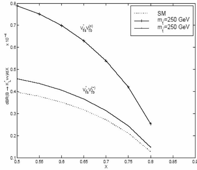
Fig. 1. The dependence of the differential of the BR of the decay B \rightarrow K^* \nu \bar{\nu} on the missing-energy fraction x at fixed value of m_t = 250 GeV when K^* is polarized longitudinally.
