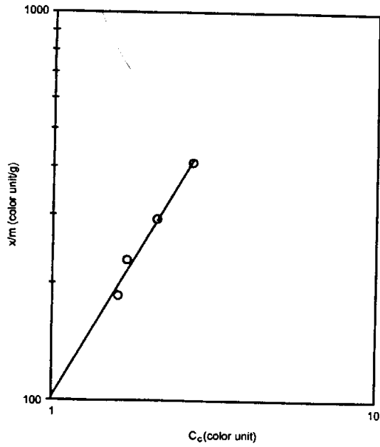
Fig. 2. Adsorption of oil color on the activated clay samples.
