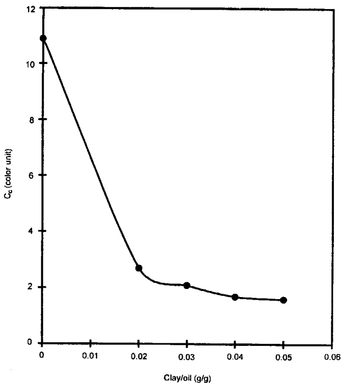
Fig. 1. Bleaching curve of oil bleached with the activated Saudi-bentonite clay.
