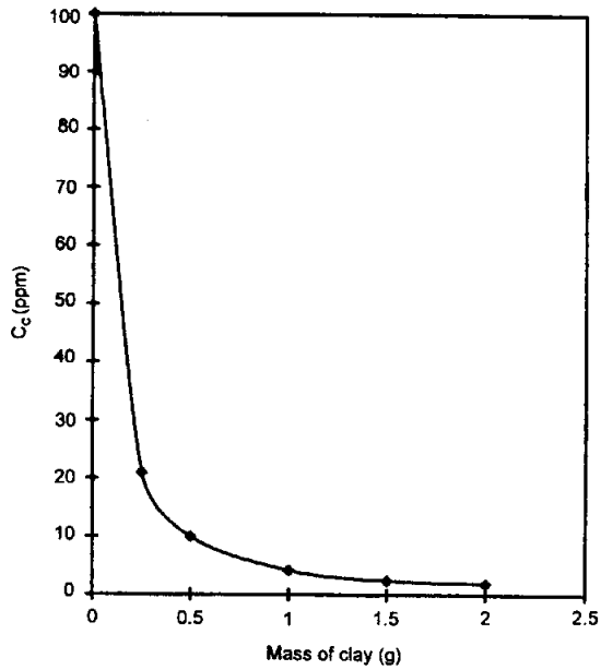
Fig. 3. Residual concentration of methyl violet as a function of clay dosage used in adsorption experiments.
