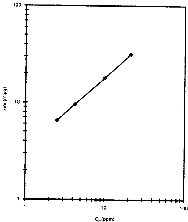
Fig. 4. Adsorption of methyl violet color on activated clay samples.
