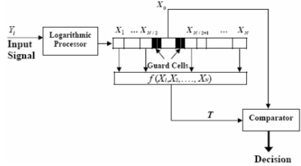
Fig. 1. Block diagram of the proposed CFAR processor.
