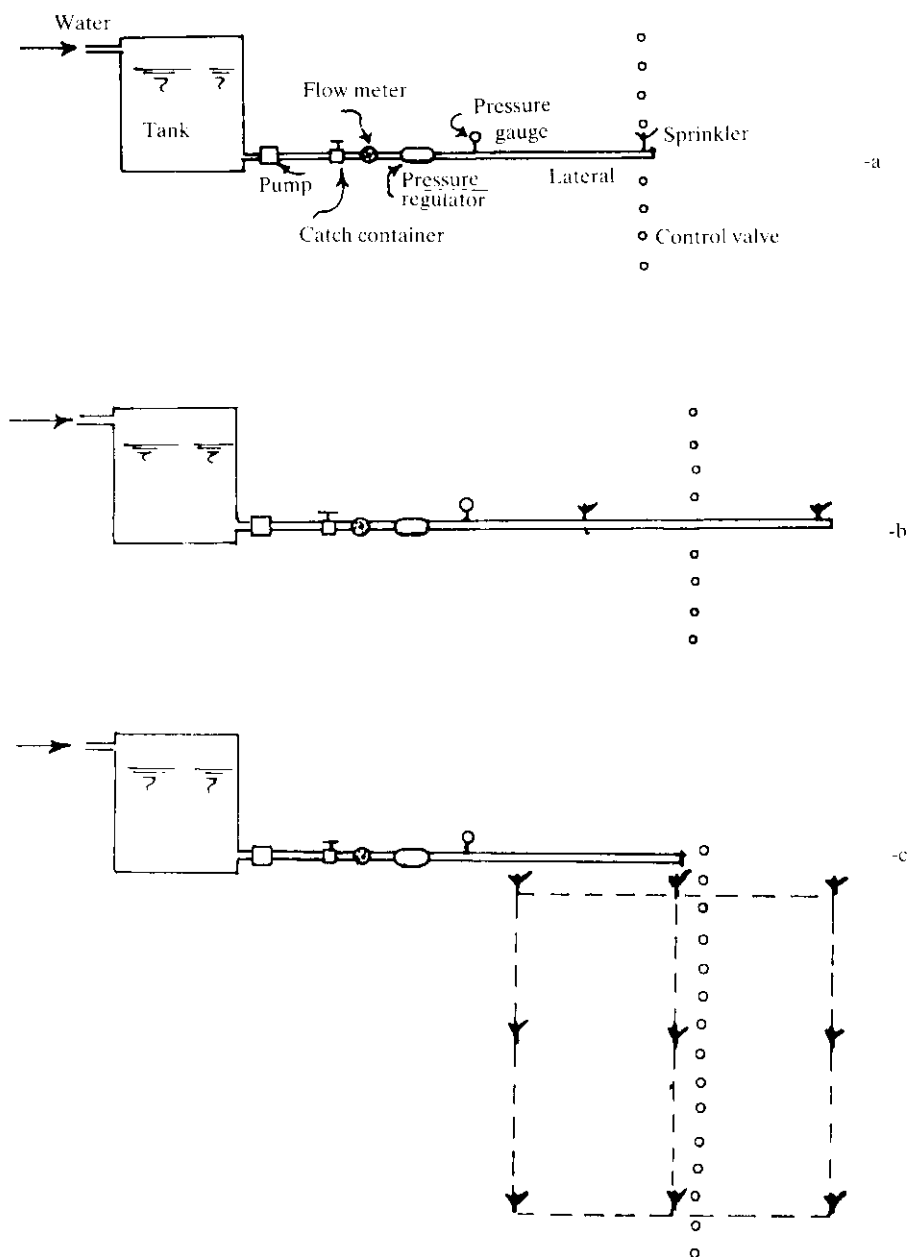
Fig. 1. Field layout of the apparatus used in the study.
