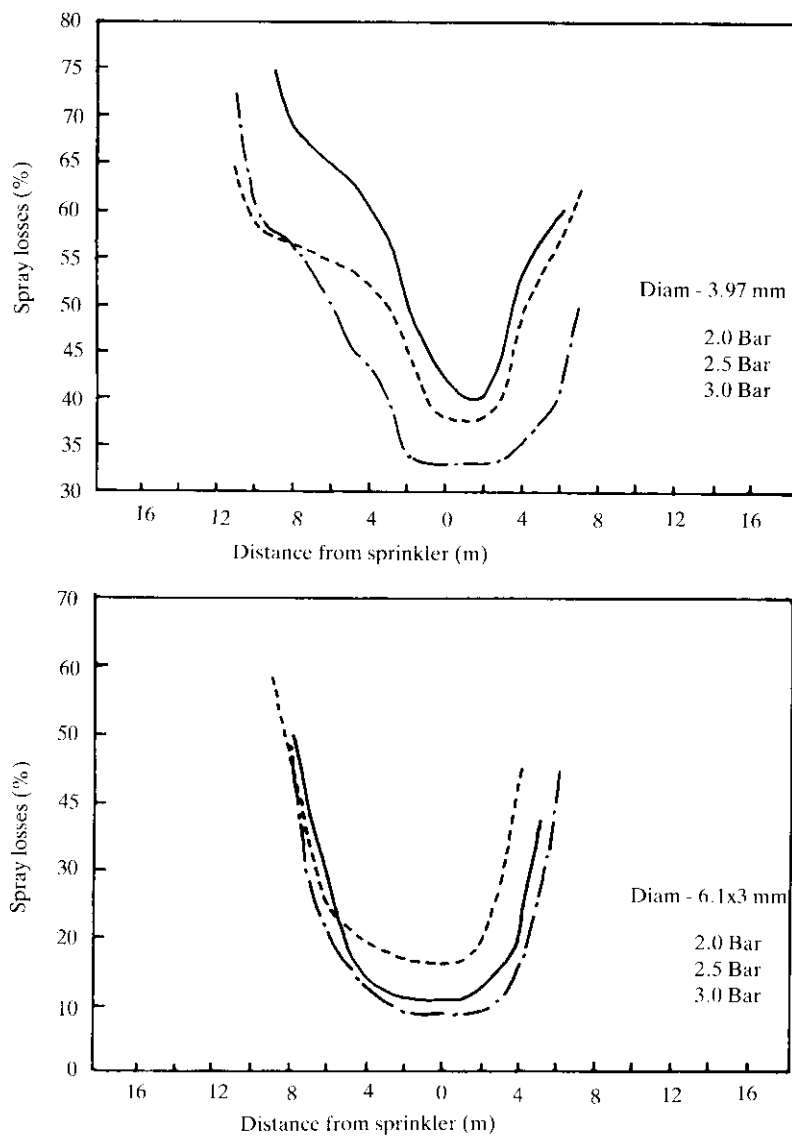
Fig. 2. Variation of spray losses with distance from a single sprinkler at different operating pressures.
