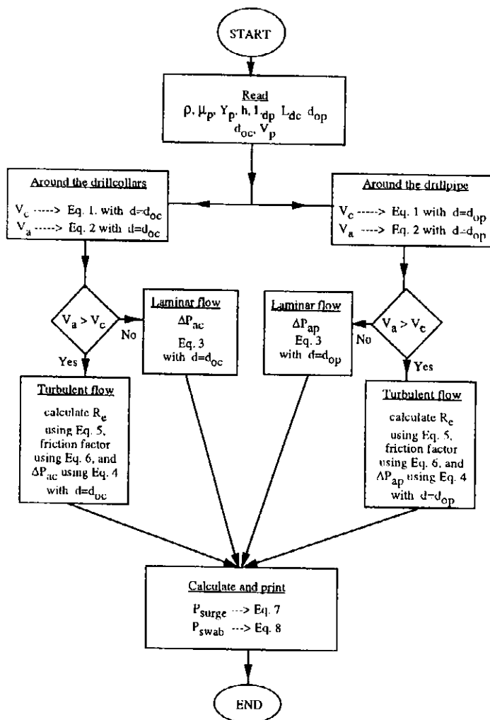
Fig. 1. Flow chart of the developed computer program.
