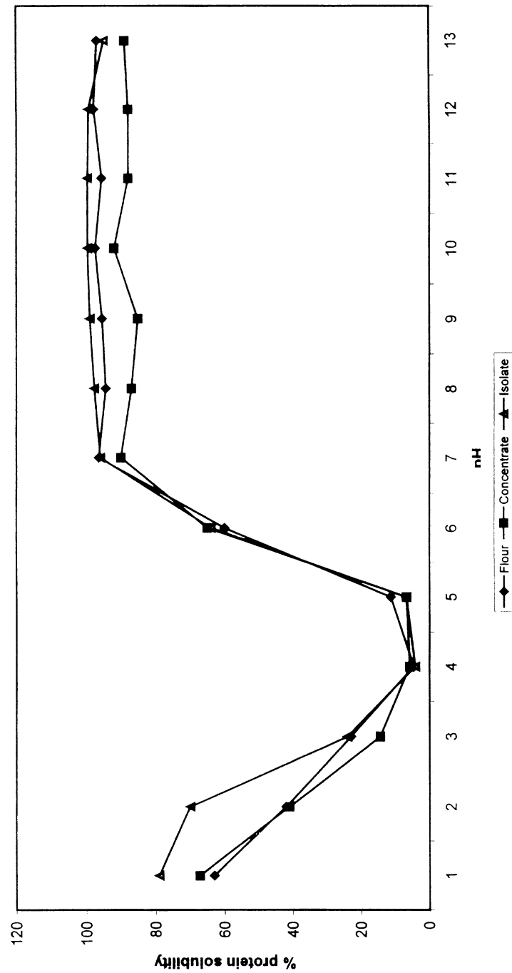
Fig. 1. Solubility profile of the flour, protein concentrate and protein isolate of lablab proteins.
