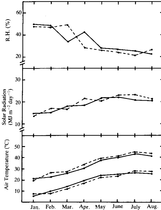
Fig. 1. Mean daily minimum and maximum air temperature, solar radiation and average relative humidity during 1987 (●-----●) and 1988 (●—●) experimental periods.
