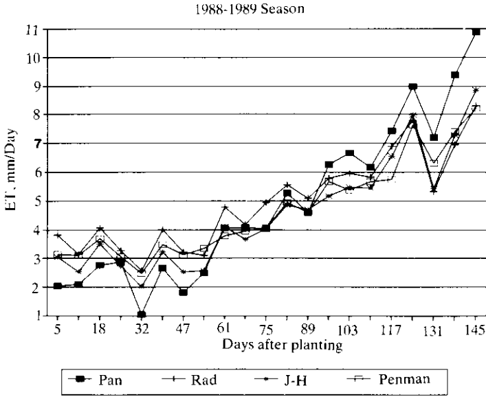
Fig. 3. Comparison of different methods of estimating daily ET_0 for 1989-1990 data.
