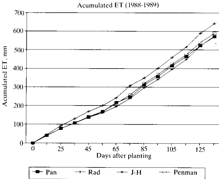
Fig. 2. Cumulative ET_0 calculated by different methods for 1988-1989 data.
