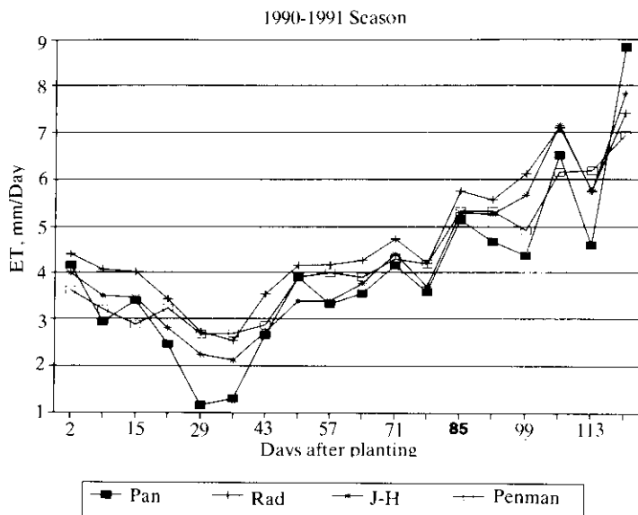
Fig. 5. Comparison of different methods of estimating daily ET 0 for 1990-1991 data.
