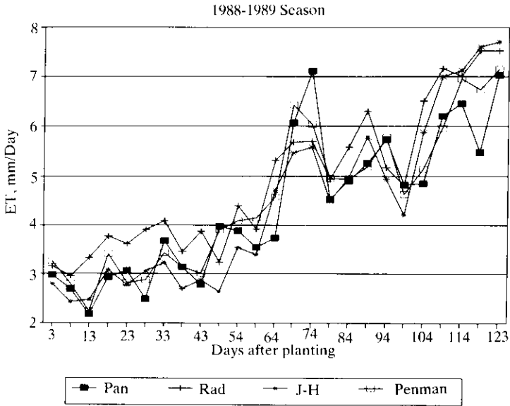
Fig. 1. Comparison of different methods of estimating daily ET_0 for 1988-1989 data.
