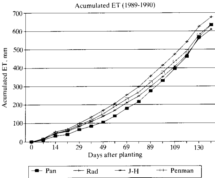
Fig. 4. Cumulative ET_0 calculated by different methods for 1989-1990 data.
