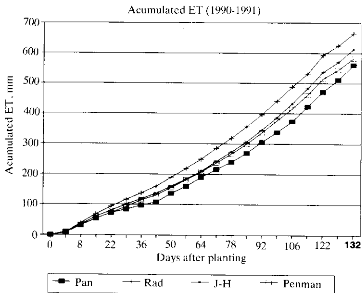
Fig. 6. Cumulative ET 0 calculated by different methods for 1990-1991 data.
