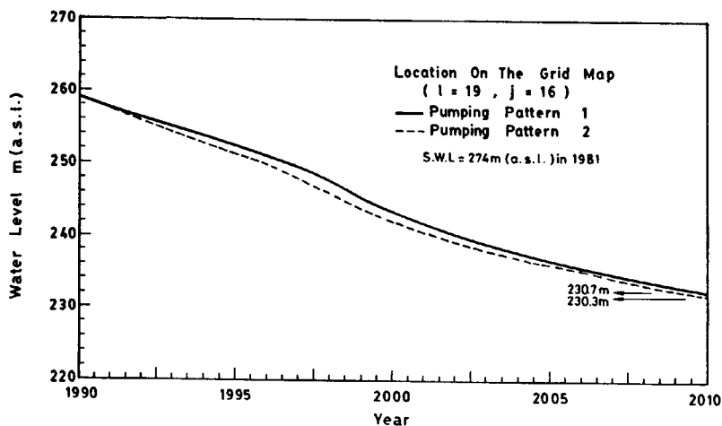
Fig. 4. Water level at the center of the well field.
