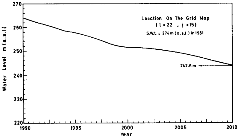
Fig. 5. Water level at the center of the well field.
