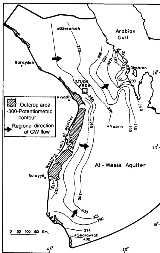
Fig. 3. Al-Wasia aquifer location.
