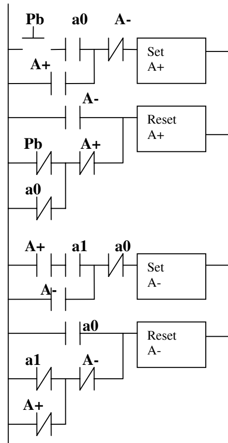
Fig. 5. Ladder diagram (C3).
