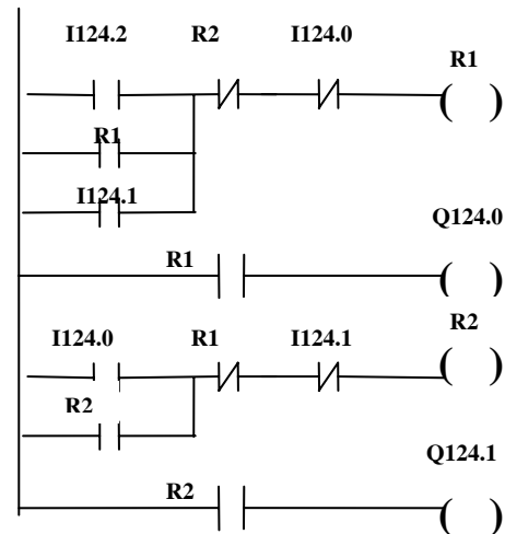
Fig.8. Ladder diagram (Design 2).
