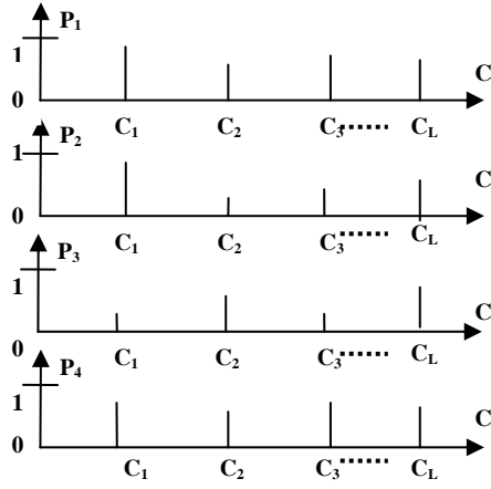
Fig. 1. Membership functions.
