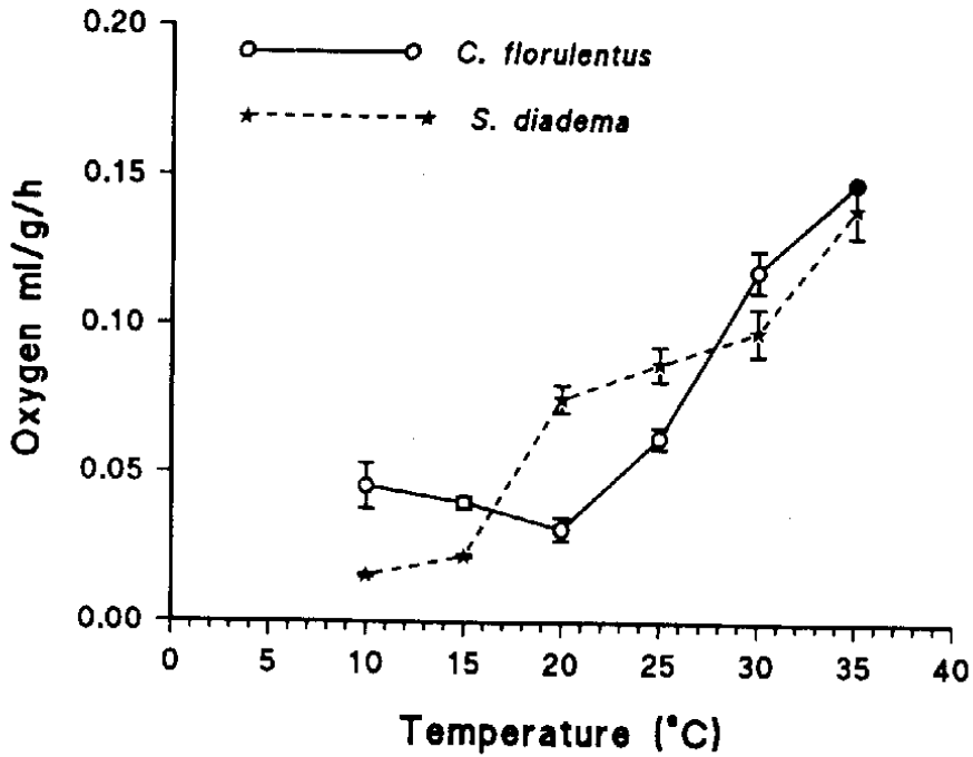
Fig. 3. Relationship between the oxygen consumption rates and the experimental temperatures of Coluber florulentus (o — o) and of Spalerosophis diadema (★-----★). [Each point represents the mean of different individual snakes. Vertical lines represent standard errors (S.E.)].
